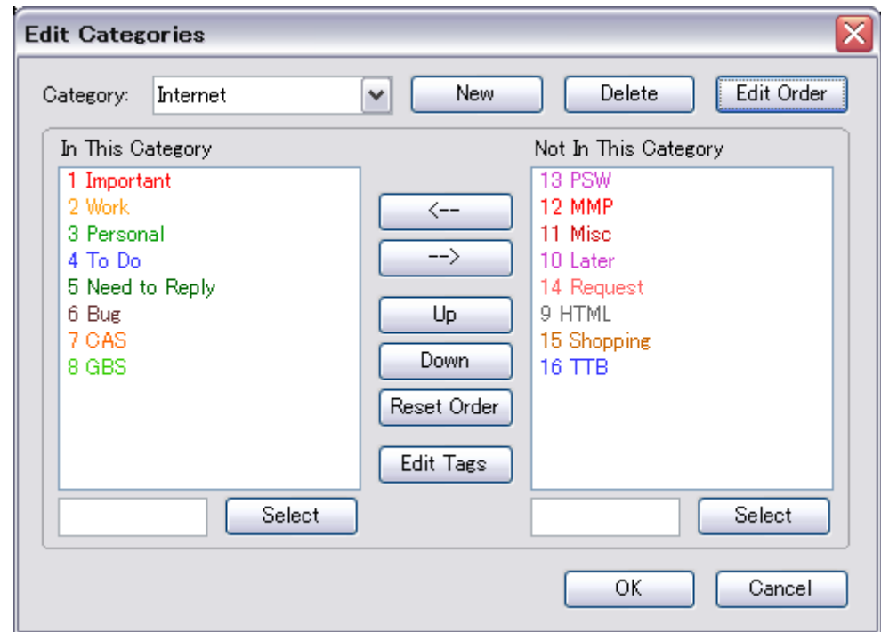
Category Editor
