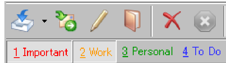
Text Mode
